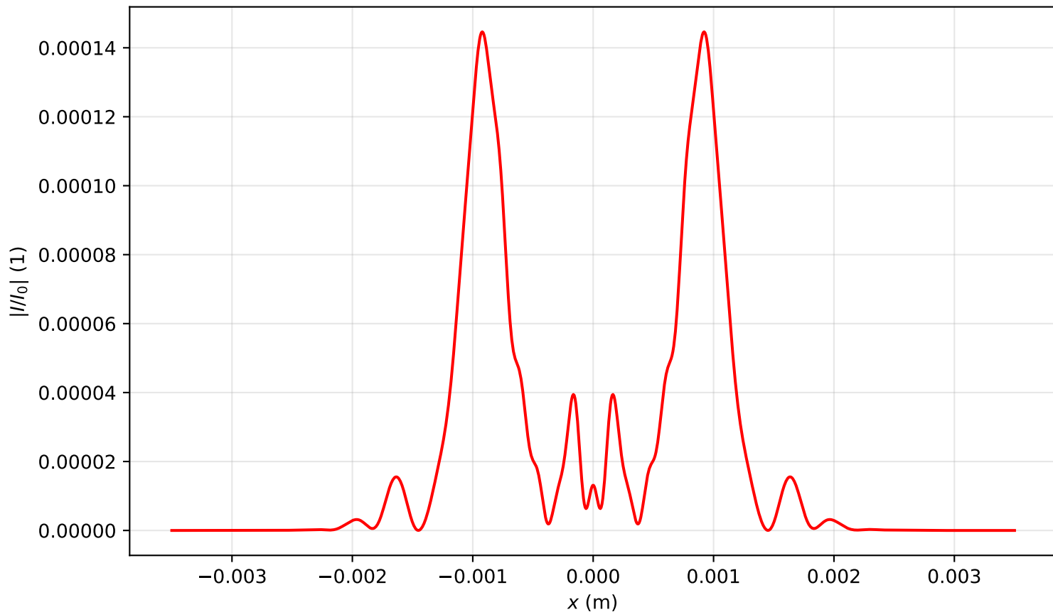
Intensity profile I(x, y = 0, z = 1.194)/I_0 , P_{in}=6.0P_{cr} , artificial time
